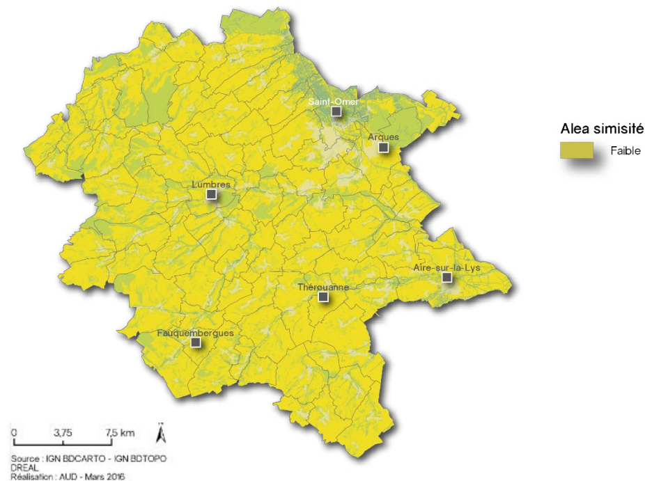
FIGURE 107. ALÉA SISMICITÉ
